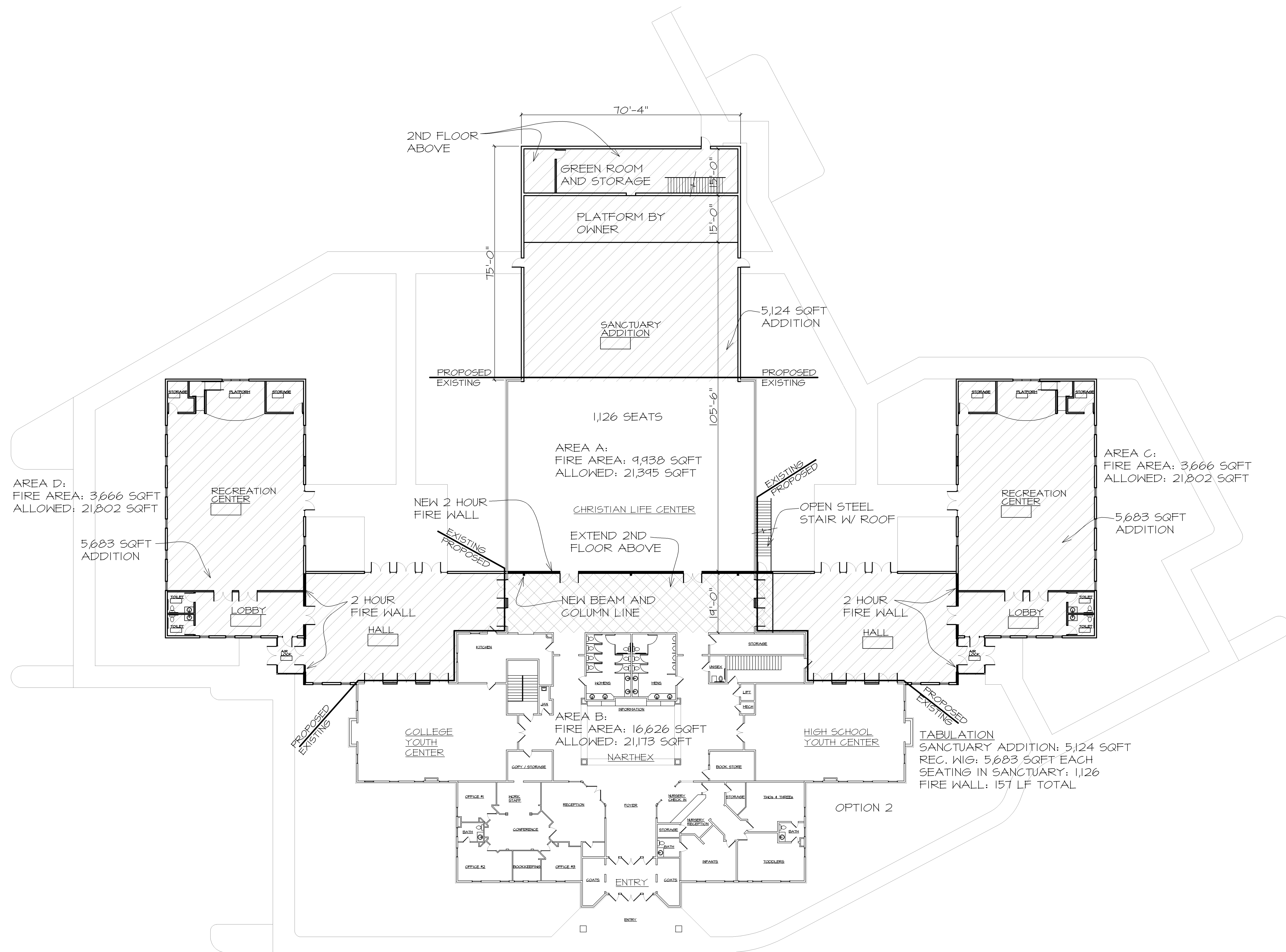
PROPOSED LAYOUT SCALE: 1/8"=1'-0"
