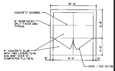
ENLARGED DUMPSTER PLAN
