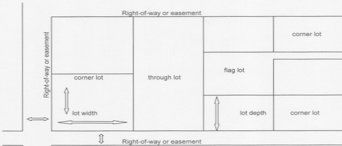
LOTS-Lot and lot line illustration
